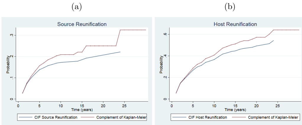
Figure C.7: CIF versus (complement of) Kaplan-Meier
