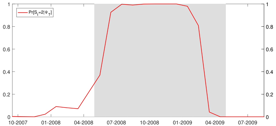
(a) MS(2)-DFM
