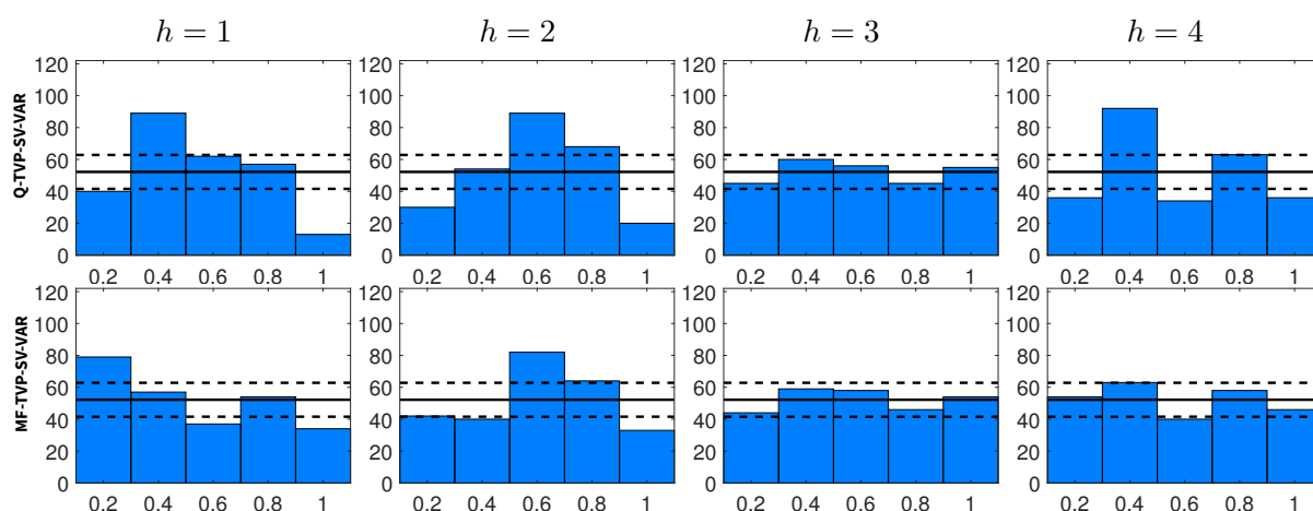
Figure 5.2 : Probability integral transforms for inflation forecasts
