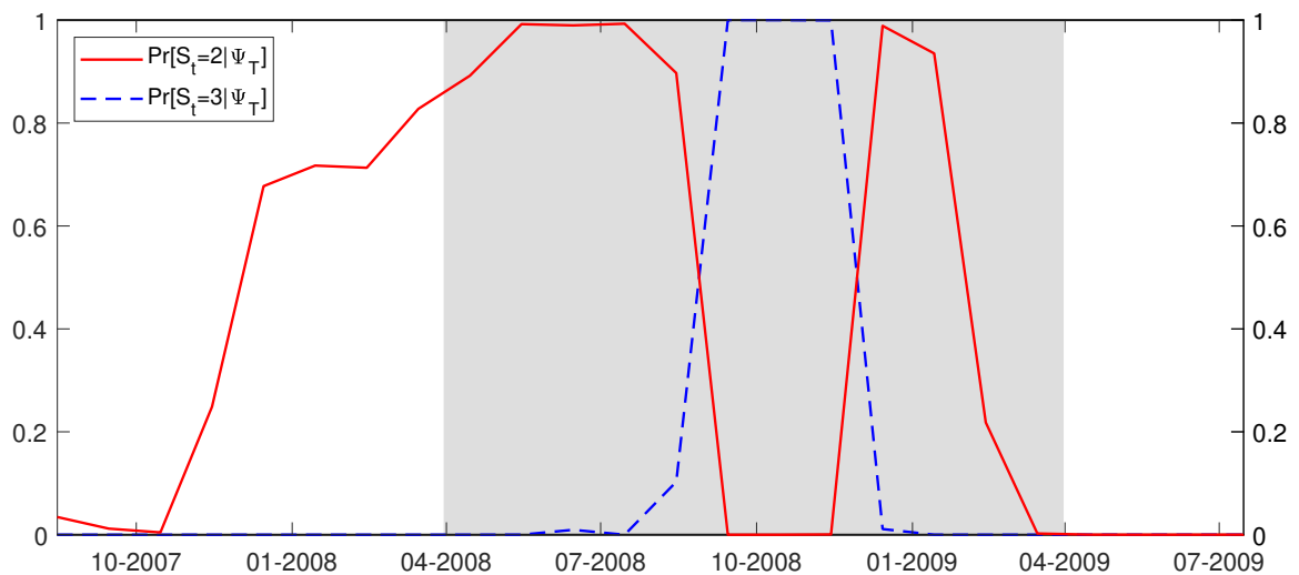
(b) MS(3)-DFM
