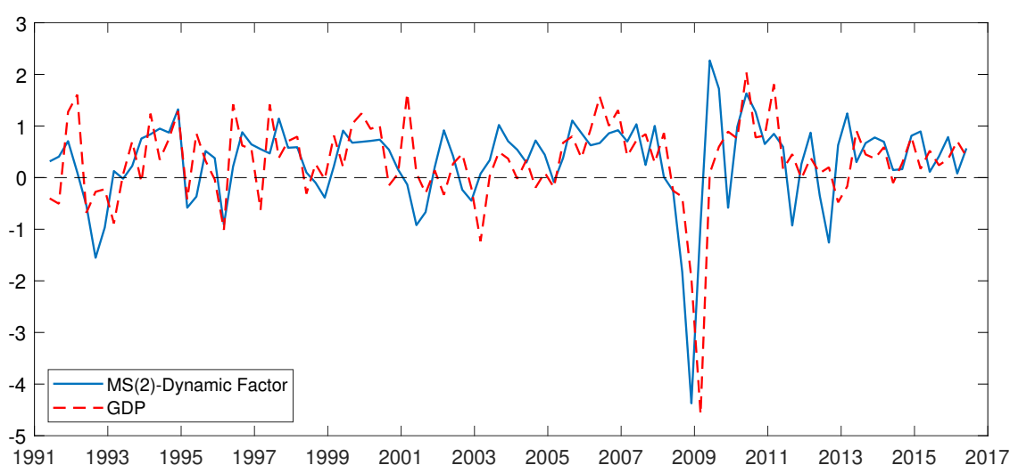
Figure 1.1 : Filtered factor of the MS(2)-DFM and GDP growth
