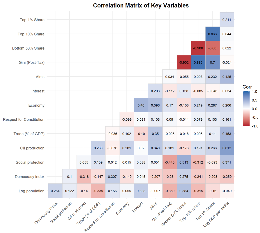
Figure 1: Correlation Matrix
